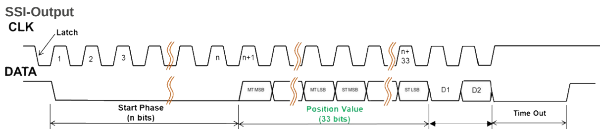
Fig. 5: By synchronous serial interface (SSI), the ASA86's encoder transfers the position values as 33-bit packets.
