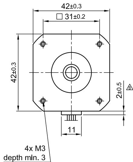
Front view and mounting
