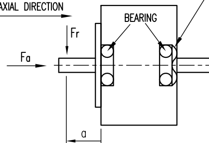
PERMISSIBLE RADIAL+AXIAL FORCE
